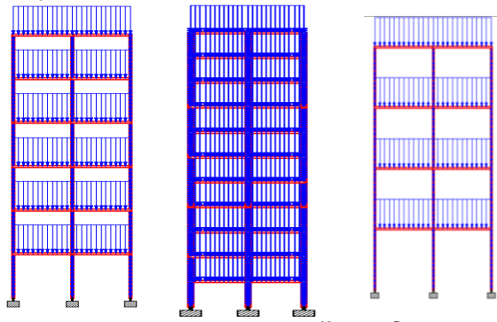
Figure 4.1: Loads taken on different Structure 5. Analysis of G+3, G+5 AND G+10 Structures on Staad Pro V8i
